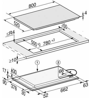
KM 7575 FL onset (installation drawing)
