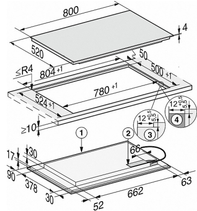
KM 7575 FL flush (installation drawing)
